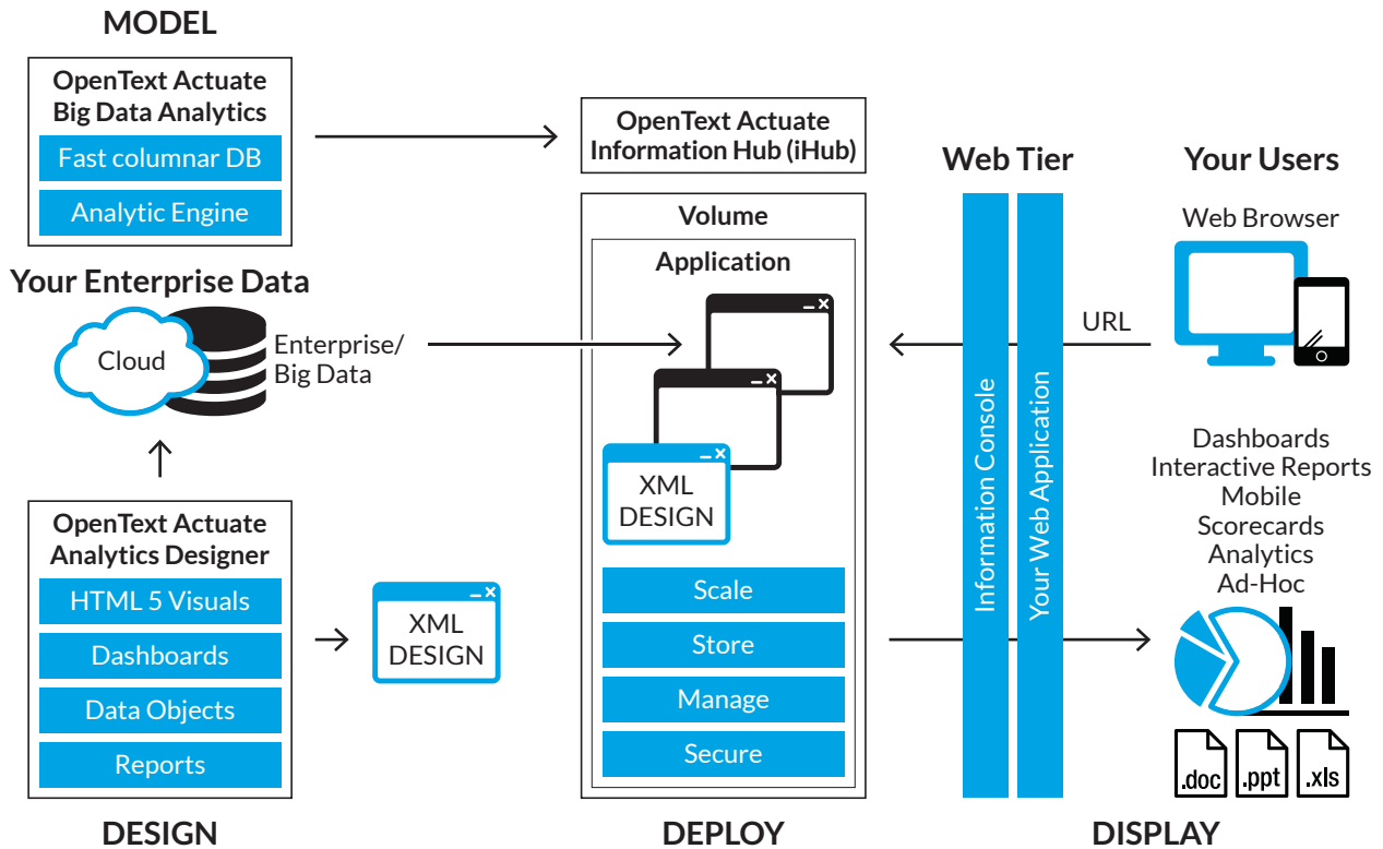
The OpenText Analytics and Reporting Information Hub Platform
